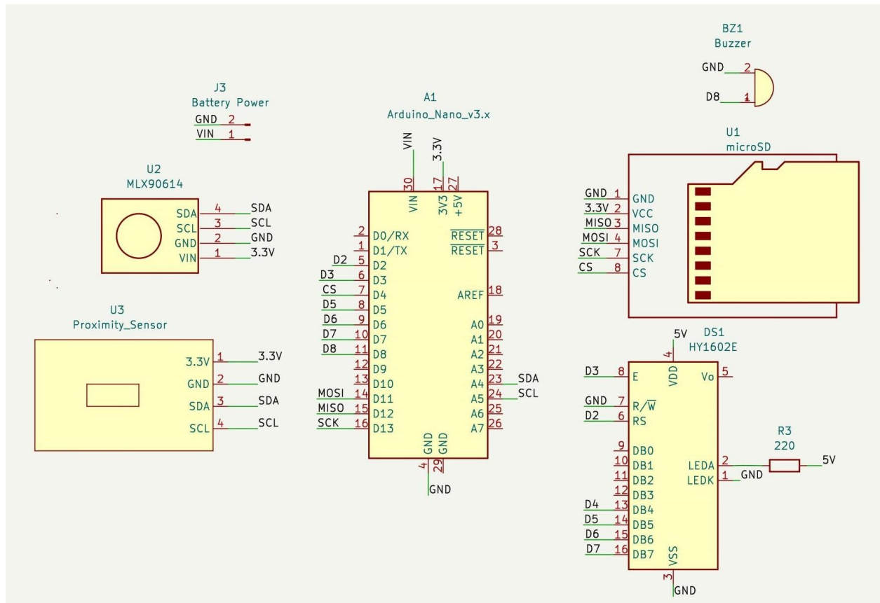
Figure 1: Electrical Schematic
