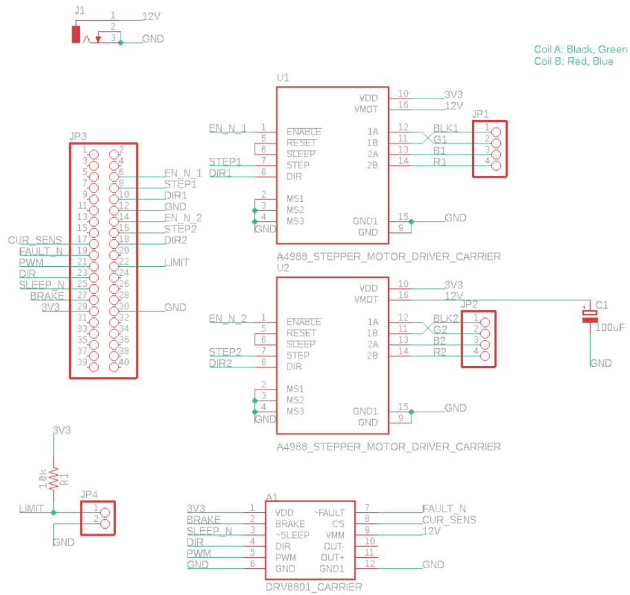
Figure 1: Schematic for stepper motor driver
