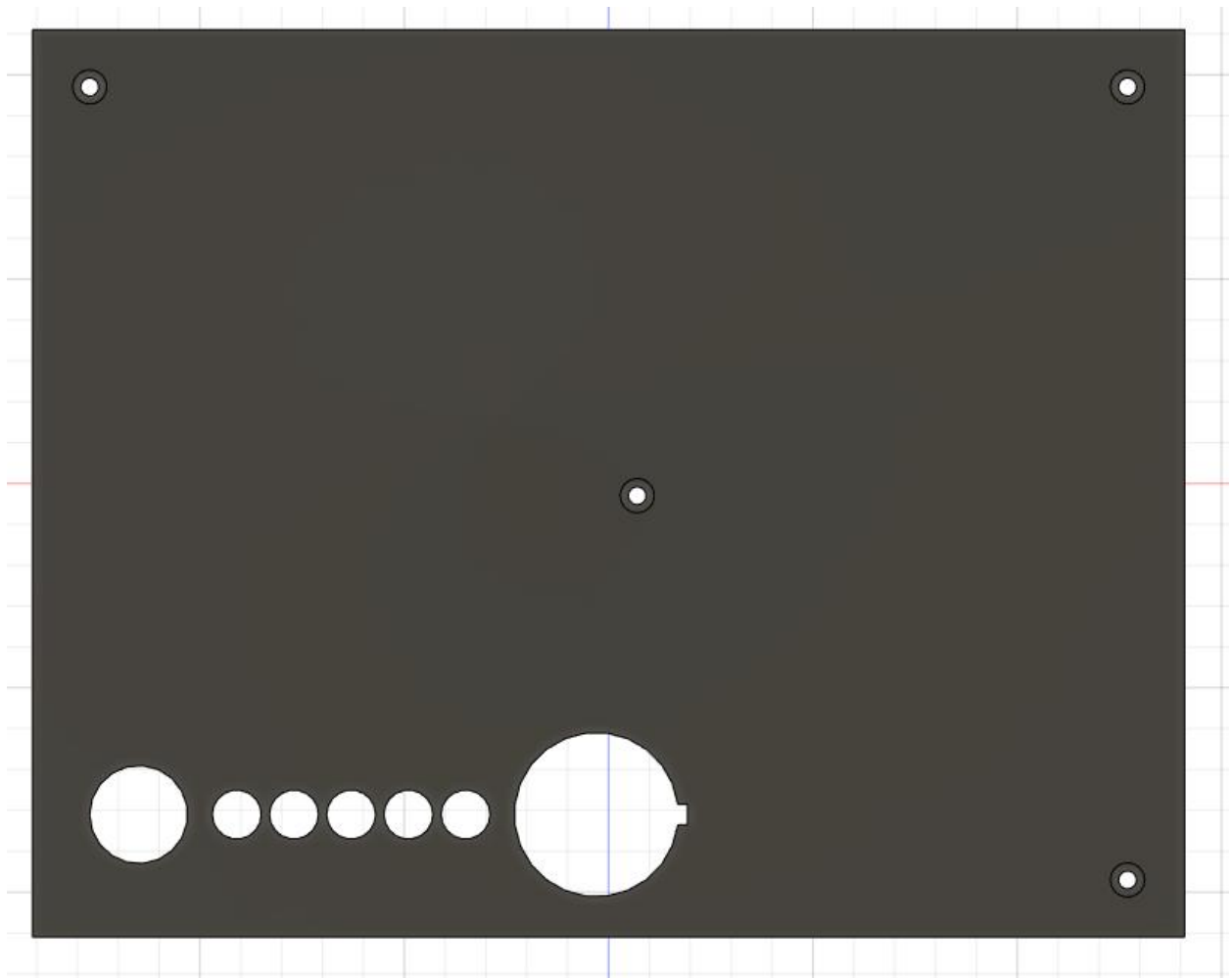
Figure 2: Enclosure Cover
