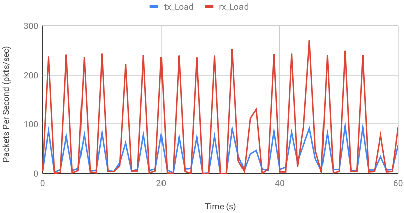
Azure VM - TX/RX Network Packet Rate (Load)
