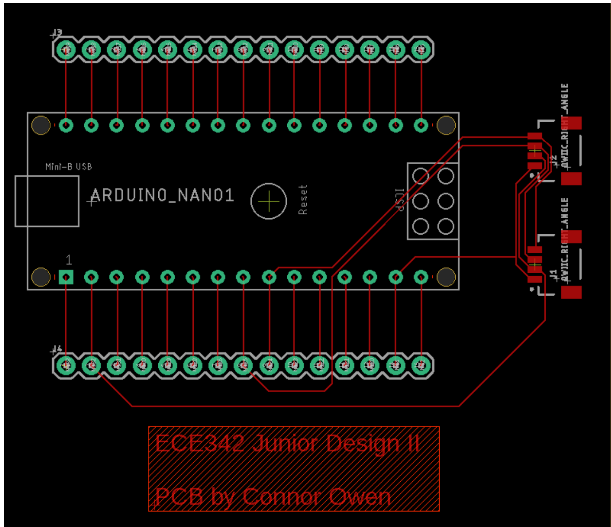
Figure 2: PCB Routing
