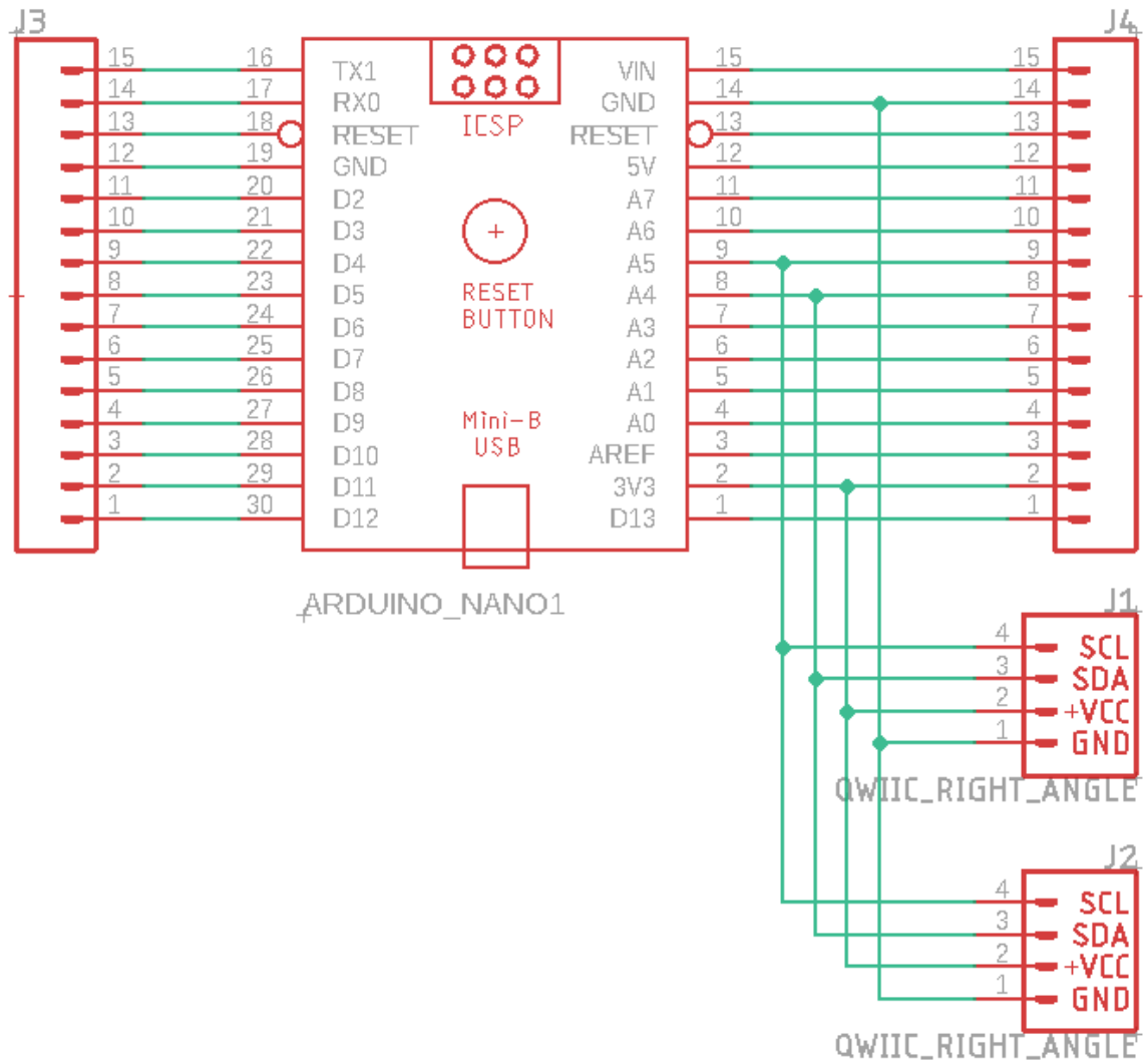
Figure 1: PCB Wiring Diagram
