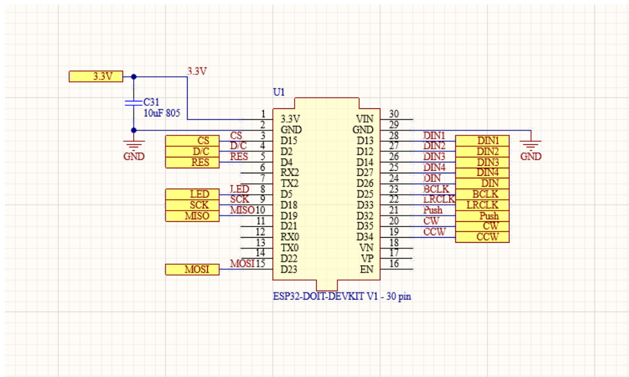
Figure 2: ESP32 Schematic
