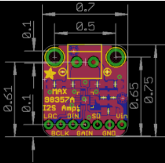
Figure 4. Adafruit PCB
