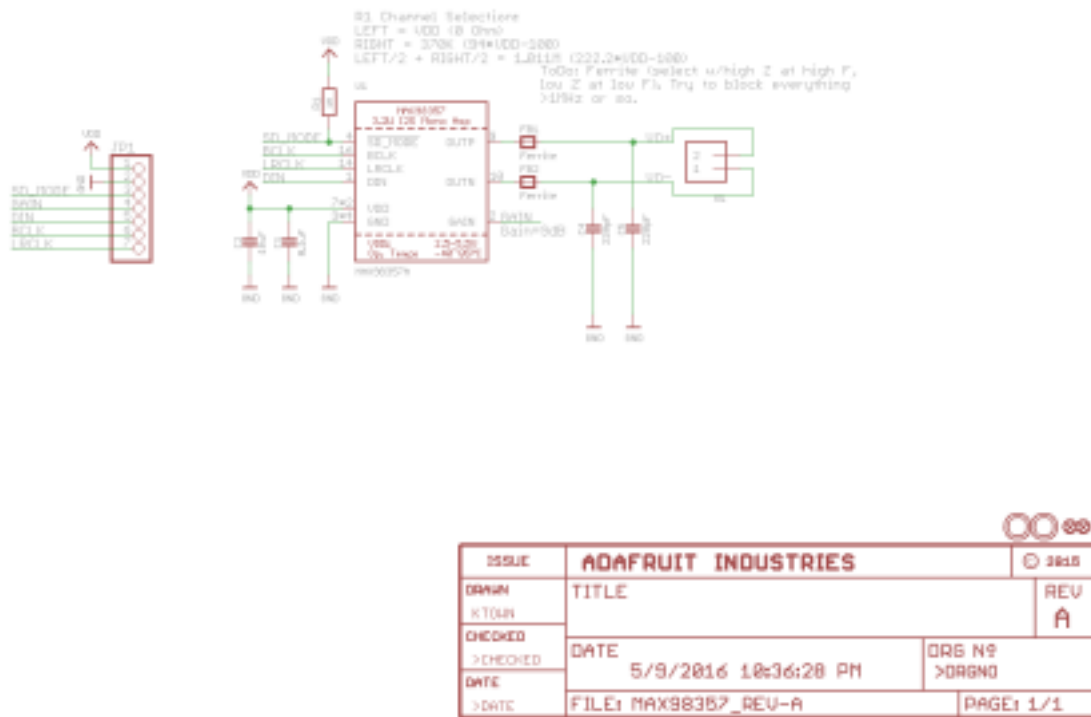
Figure 3. Adafruit Schematic
