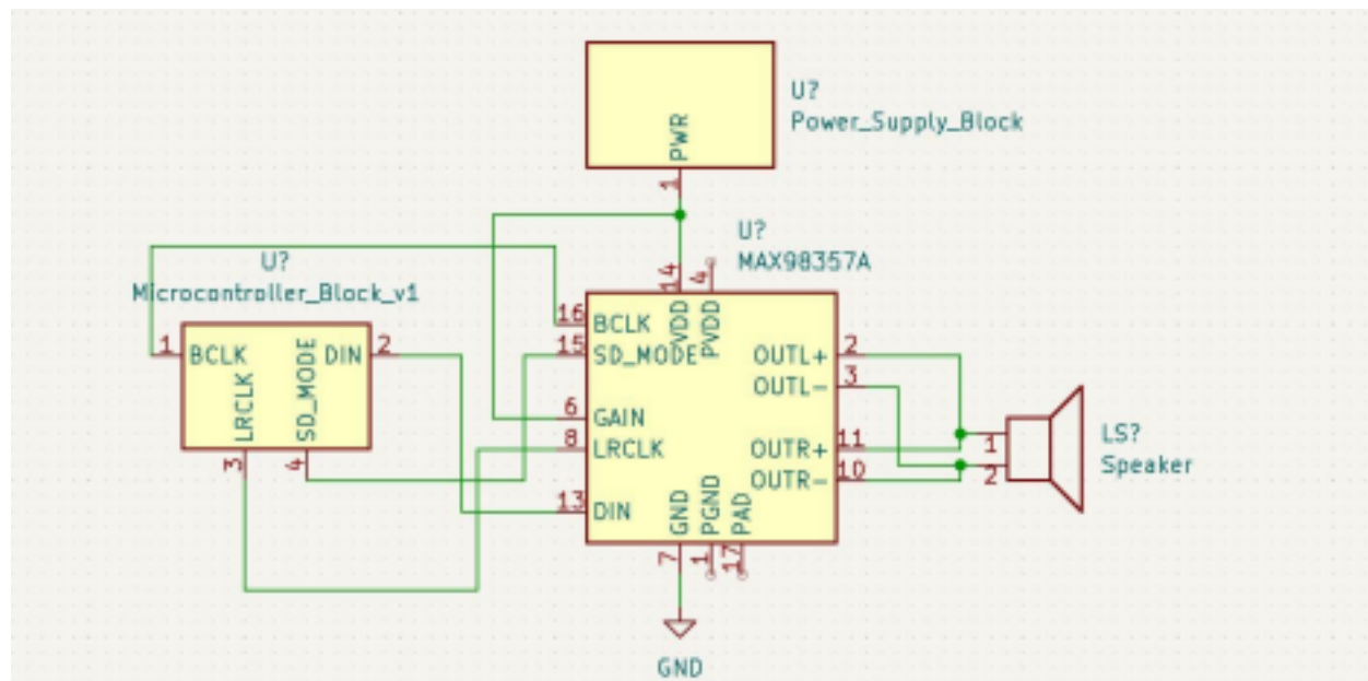
Figure 2. Block schematic
