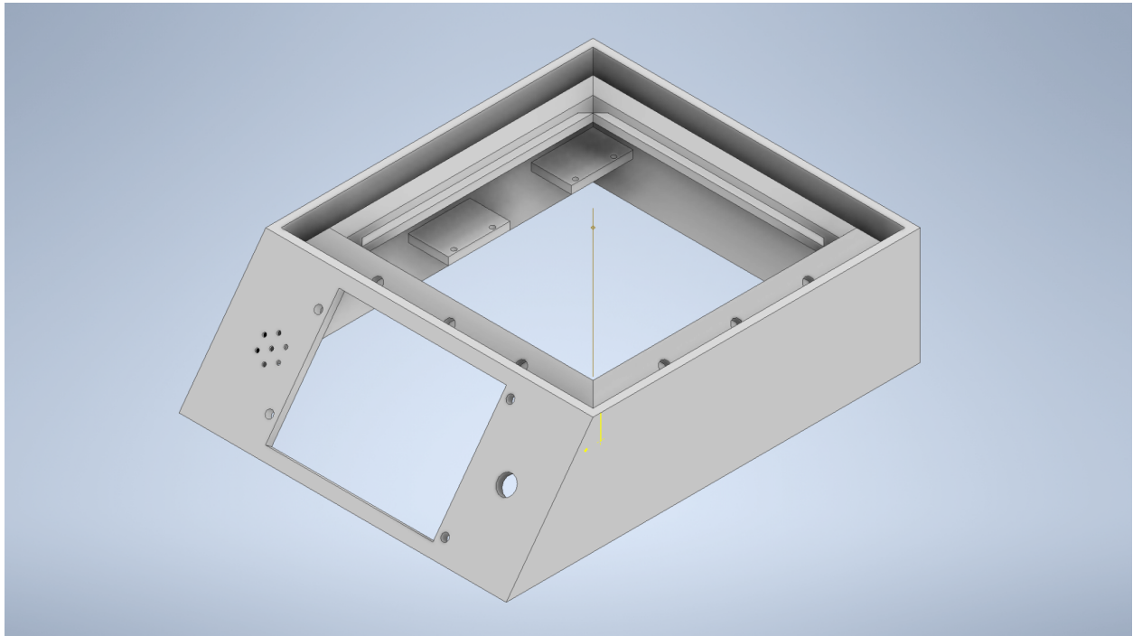
Figure 7: Enclosure Base
