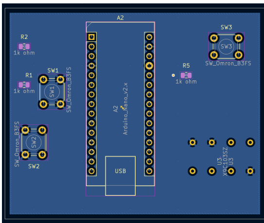
Back face (B.Cu) - Gnd
