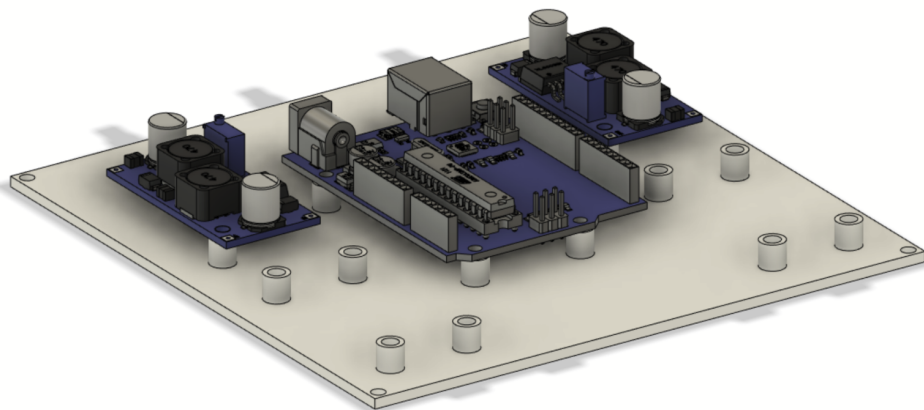
Mechanical Drawings - Baseplate
