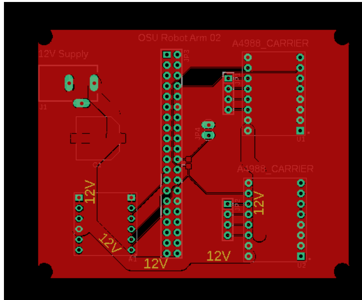
Figure 3: Top layer and silkscreen
