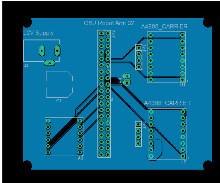
Figure 5: Bottom layer and silkscreen
